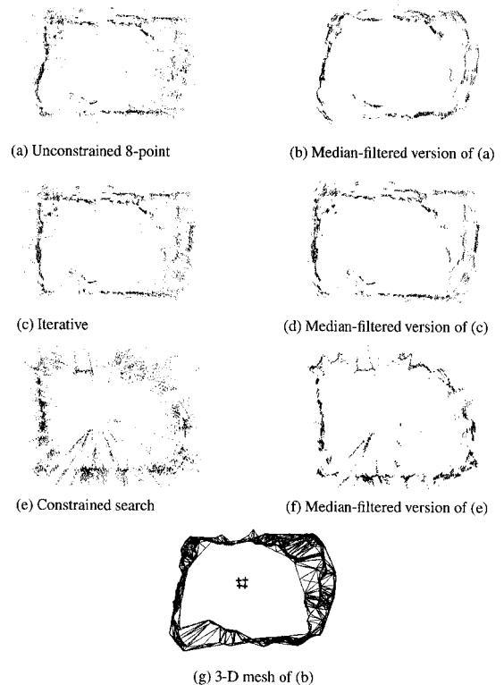
Figure 11. Extracted 3-D points and mesh of office scene. Notice that the recovered distributions shown in (c) and (d) appear more rectangular than those shown in (a) and (b). The camera locations are indicated by +'s in (g).
