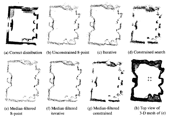
Figure 8. Comparison of 3-D points recovered of synthetic room. The four camera locations are indicated by +’s in (h).
