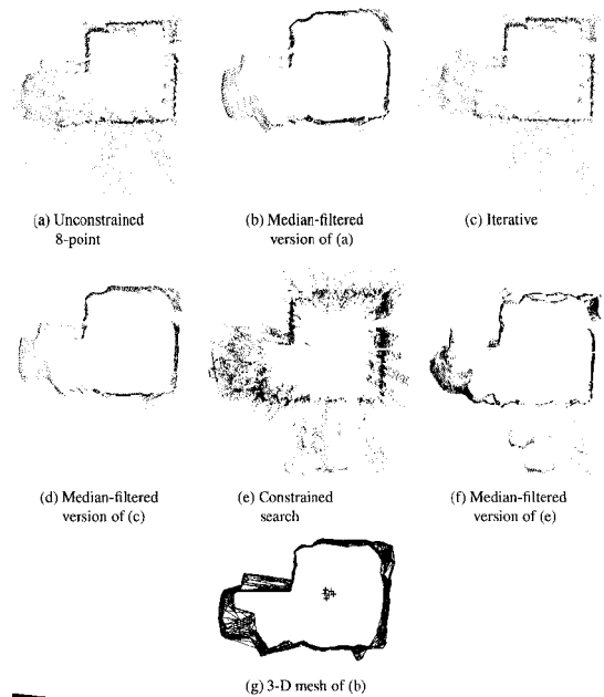
Figure 14. Extracted 3-D points and mesh of laboratory scene. The camera locations are indicated by +’s in (g).
