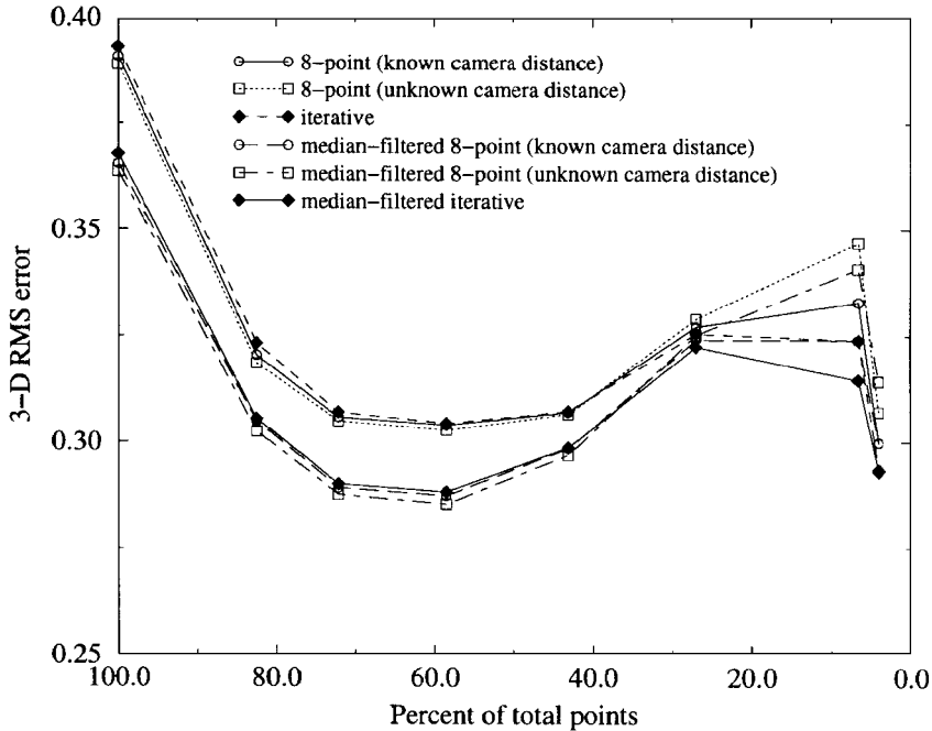
Figure 10. 3-D RMS error vs. number of points. The original number of points (corresponding to 100%) is 3057. The dimensions of the synthetic room are 10 (length) \times 8 (width) \times 6 (height). Note that by “8-point”, we mean the reconstruction method 1, with the application of the 8-point algorithm and direct 3-D position calculation. The “iterative” method is reconstruction method 2. The results of reconstruction method 3 is not represented here because the selected points (2-D location and sample size) are different.
