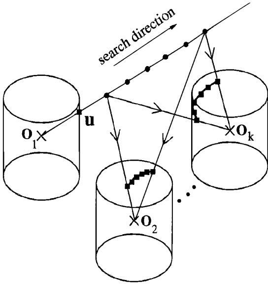
Figure 6. Principle of omnidirectional multibaseline stereo. O_1 \dots O_k represent the centers of the panoramic images 1 to k , respectively, with panoramic image 1 taken to be the reference image.
