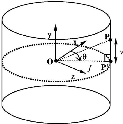
Figure 5. Cylindrical coordinate system. \mathbf{P} is any point on the cylindrical surface while \mathbf{P}' is the point projected on the x - z plane. \theta is the angle subtended by the x -axis and the line segment \mathbf{O}\text{-}\mathbf{P}' , \mathbf{O} being the center of the coordinate frame. f is the camera focal length while v is the height of point \mathbf{P} .
