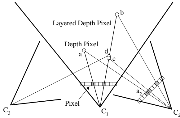
Figure 5 Layered Depth Image
